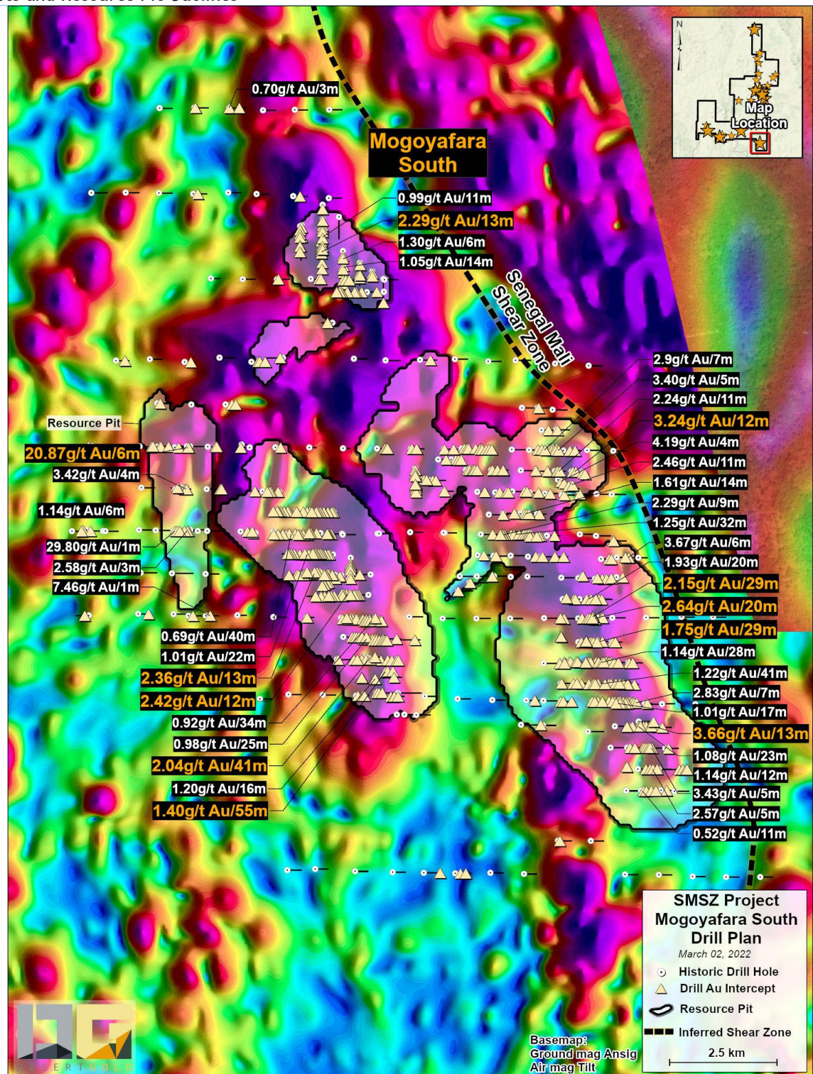
Figure 51: Mogoyafara South Deposit Area with Ground Magnetic Base, Significant Drill Results, Drill Intercepts and Resource Pit Outlines
