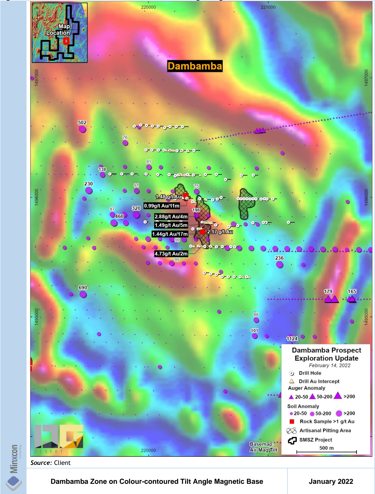
Figure 45: Dambamba Zone on Colour-contoured Tilt Angle Magnetic Base
