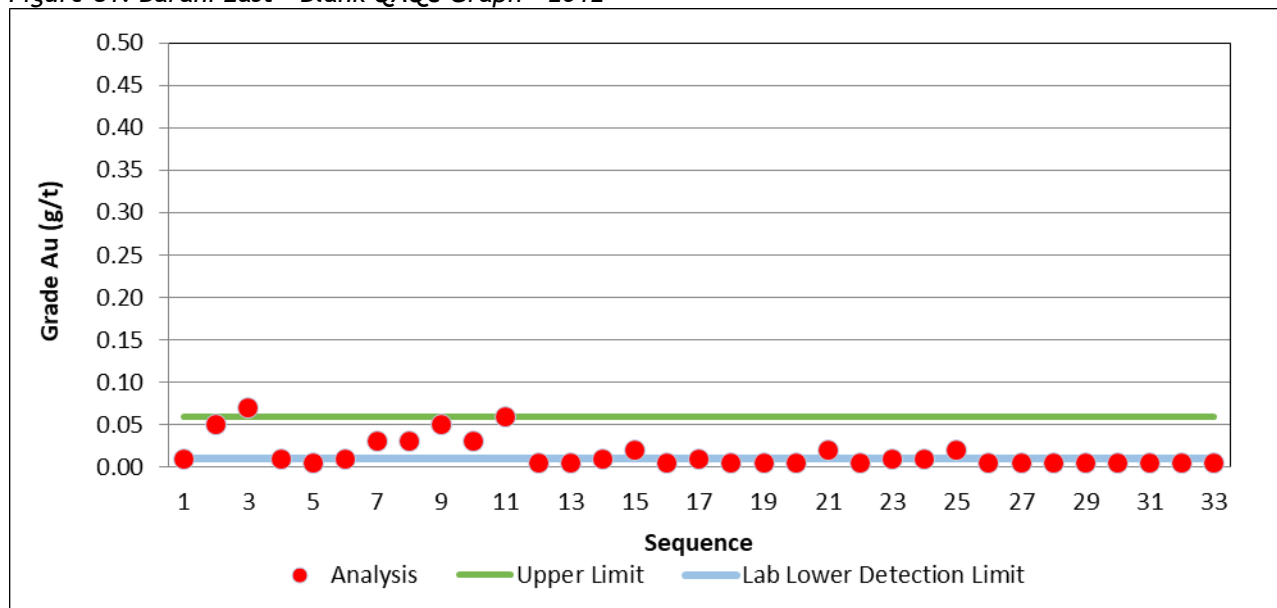
Figure 81: Barani East - Blank QAQC Graph - 2012
