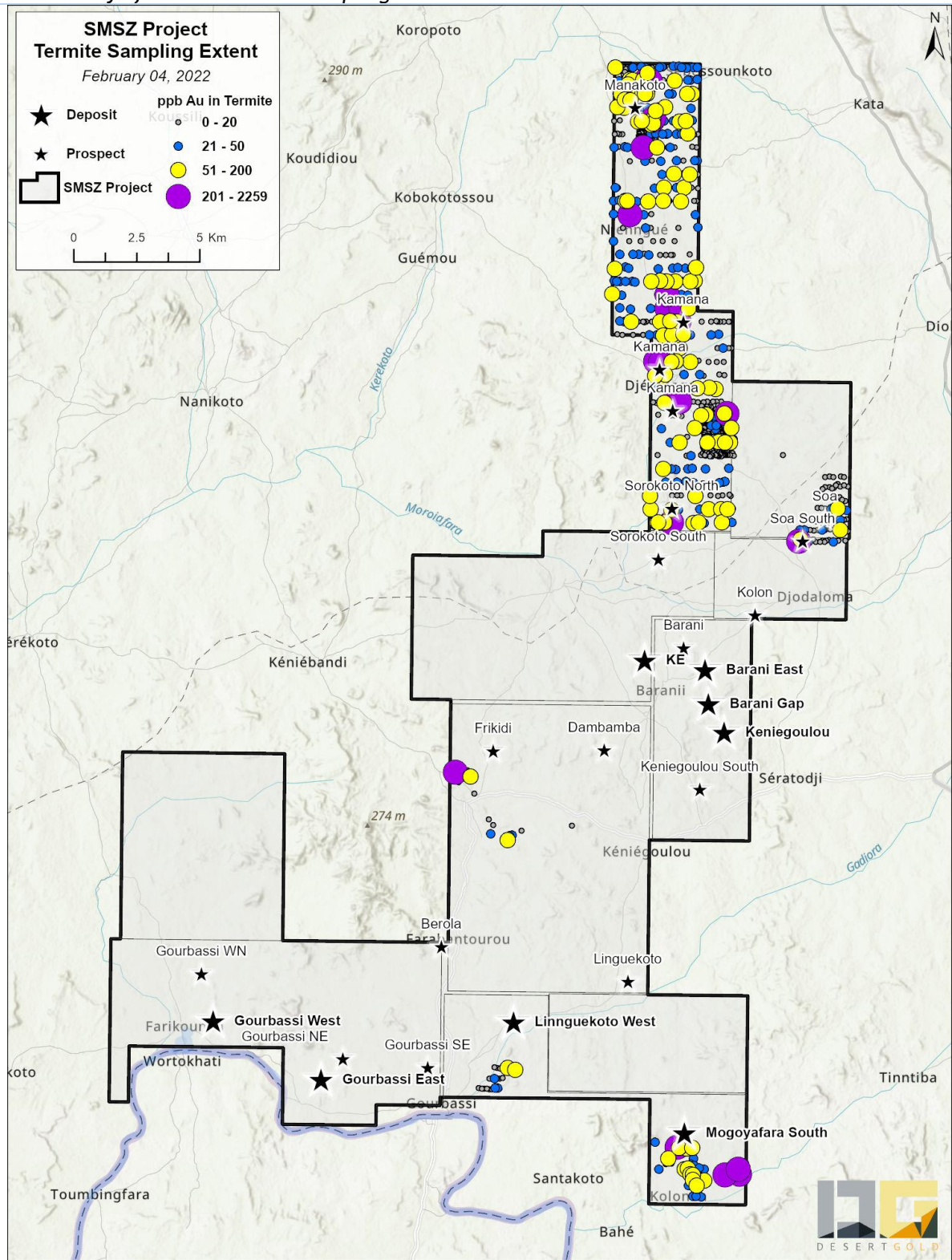
Figure 30: Summary of Termite Mound Sampling Results
