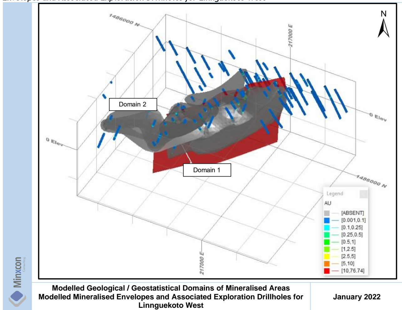
Figure 128: Modelled Geological / Geostatistical Domains of Mineralised Areas Modelled Mineralised Envelopes and Associated Exploration Drillholes for Linnguekoto West
