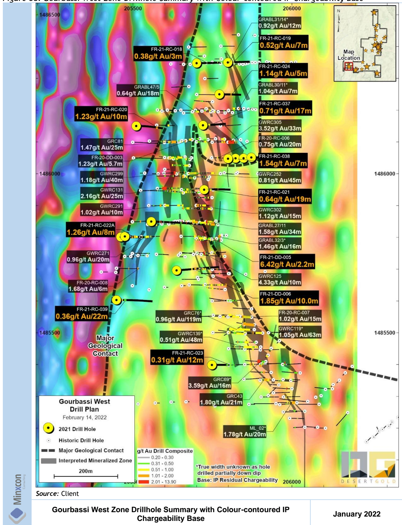
Figure 58: Goubassi West Zone Drillhole Summary with Colour-contoured IP Chargeability Base
