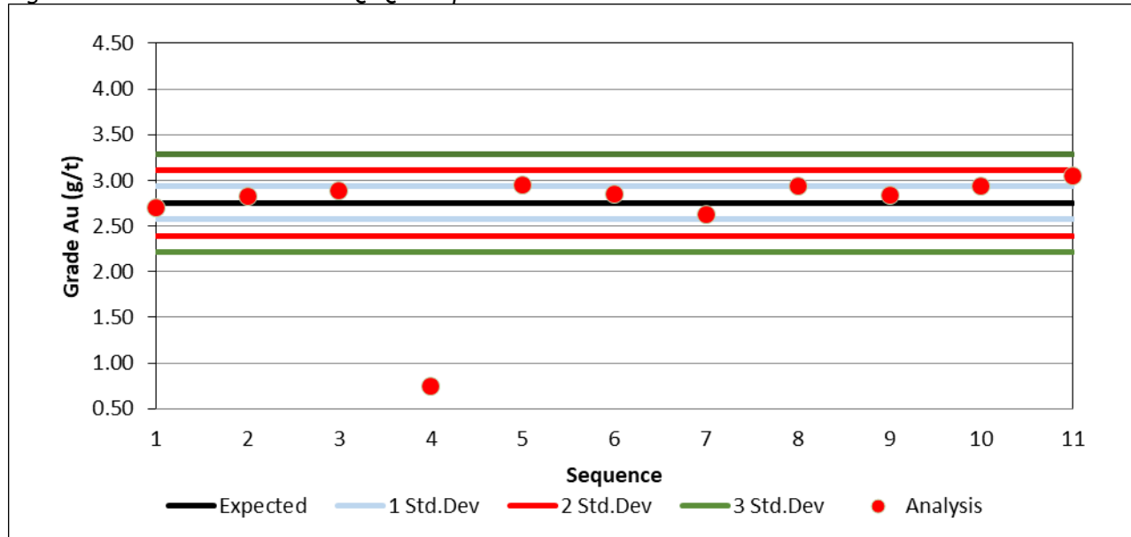
Figure 78: Barani East - G995-1 QAQC Graph - 2012
