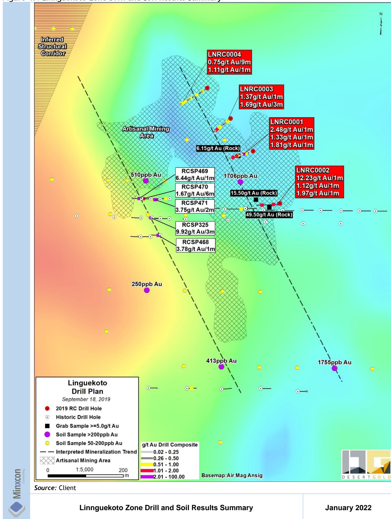
Figure 49: Linnguekoto Zone Drill and Soil Results Summary
