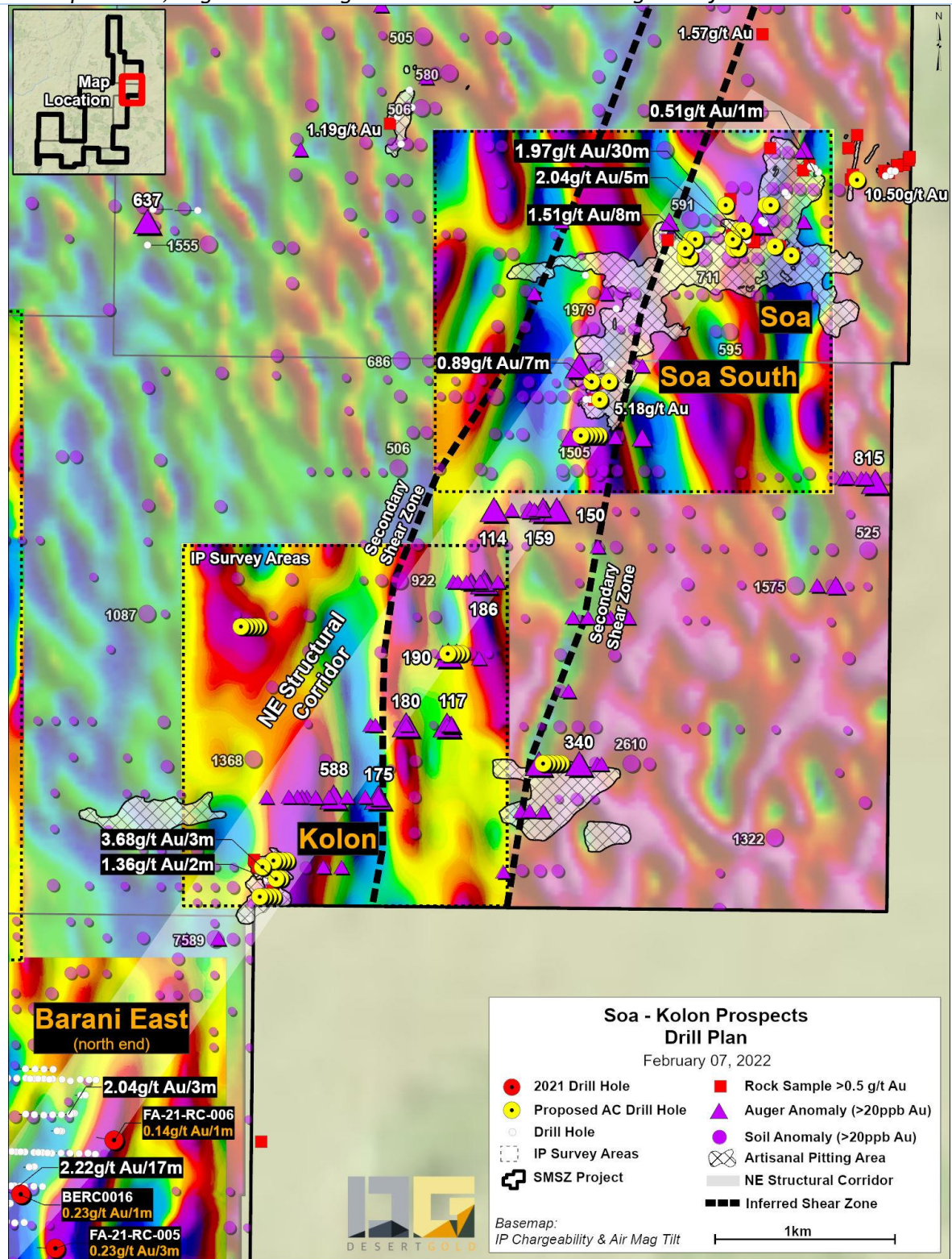
Figure 40: Compiled Soil, Auger and Drilling on Colour-contoured IP Chargeability
