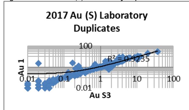
Figure 100: 2017 Au (S) Laboratory Replicates
