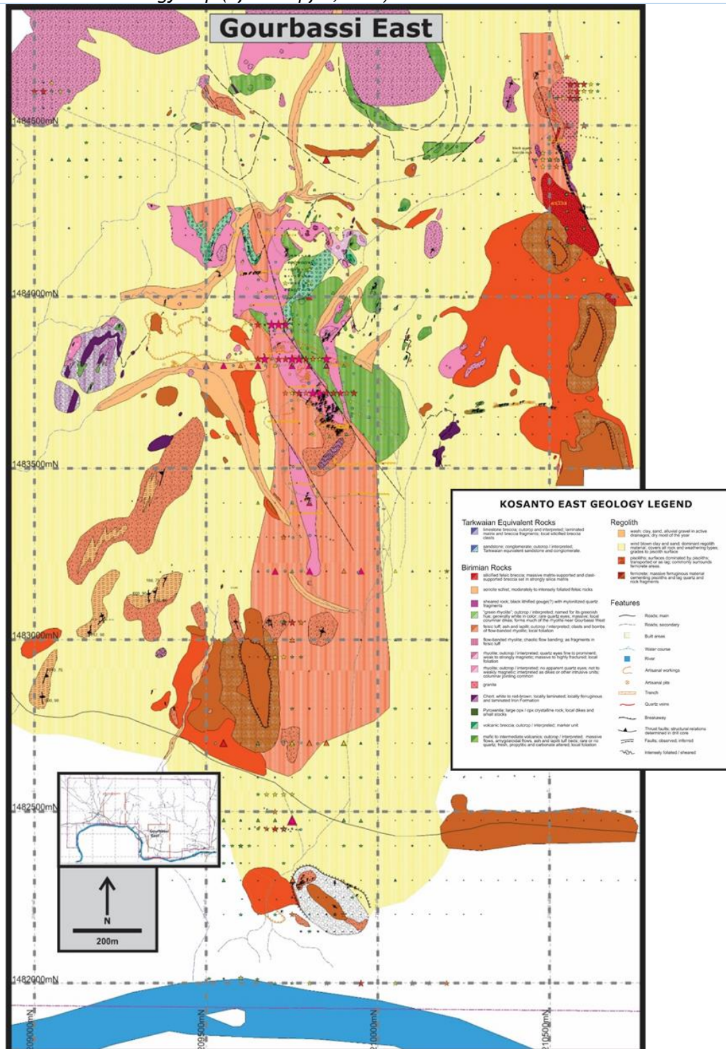
Figure 17: Gourbassi East Geology Map (after Klipfel, 2019)
