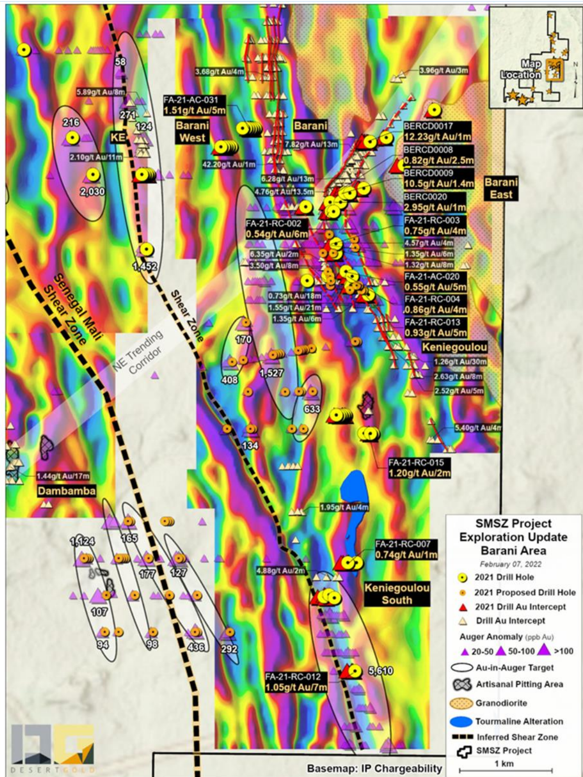
Figure 42: Barani, Keniegoulou, Barani East Area Results Summary on Colour-contoured IP Chargeability Map
