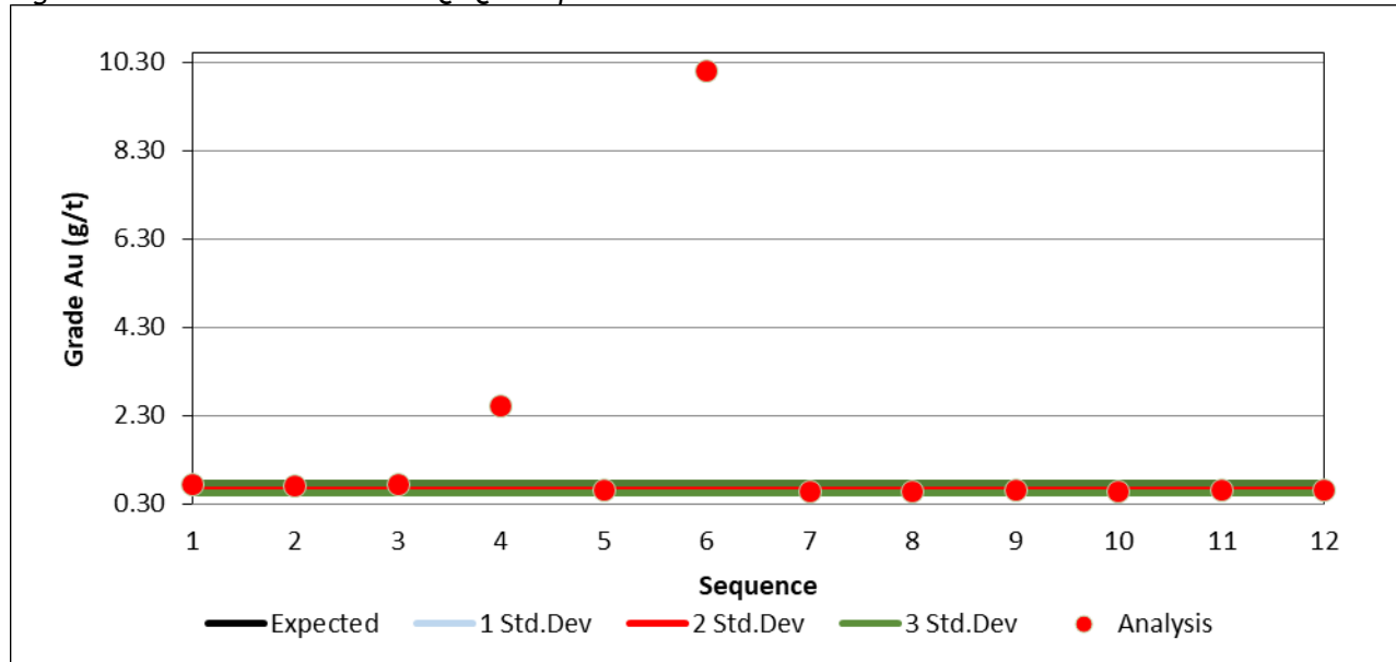
Figure 80: Barani East - G310-6 QAQC Graph - 2012
