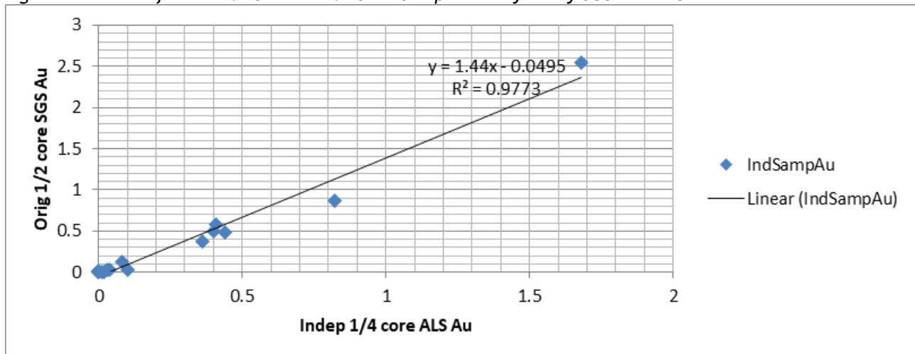
Figure 101: Plot of Paired \frac{1}{2} Core and \frac{1}{4} Core Samples Analysed by SGS and ALS
