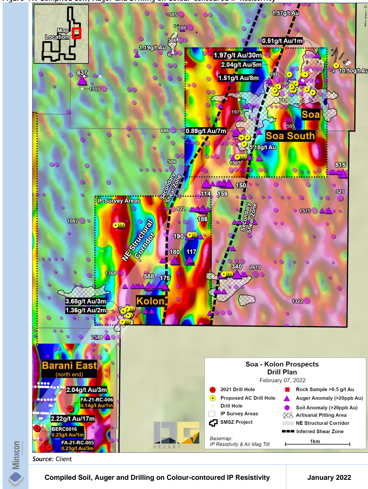
Figure 41: Compiled Soil, Auger and Drilling on Colour-contoured IP Resistivity
