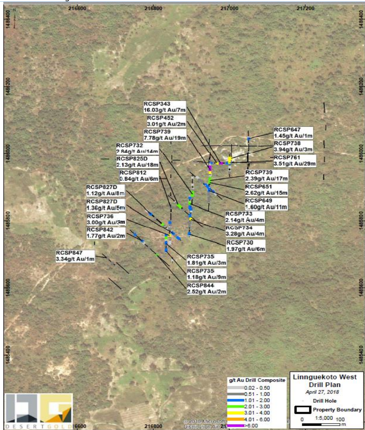
Figure 53: Plan View Linnguekoto West Zone
