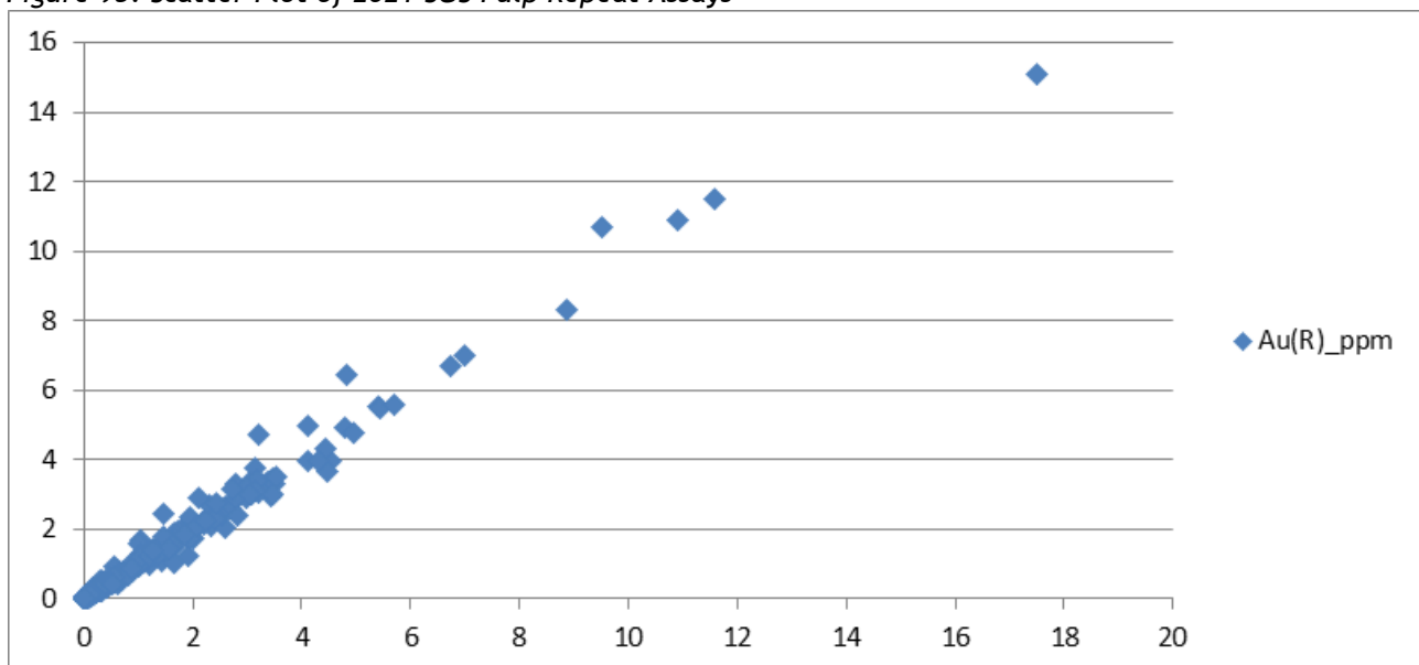
Figure 95: Scatter Plot of 2021 SGS Pulp Repeat Assays
