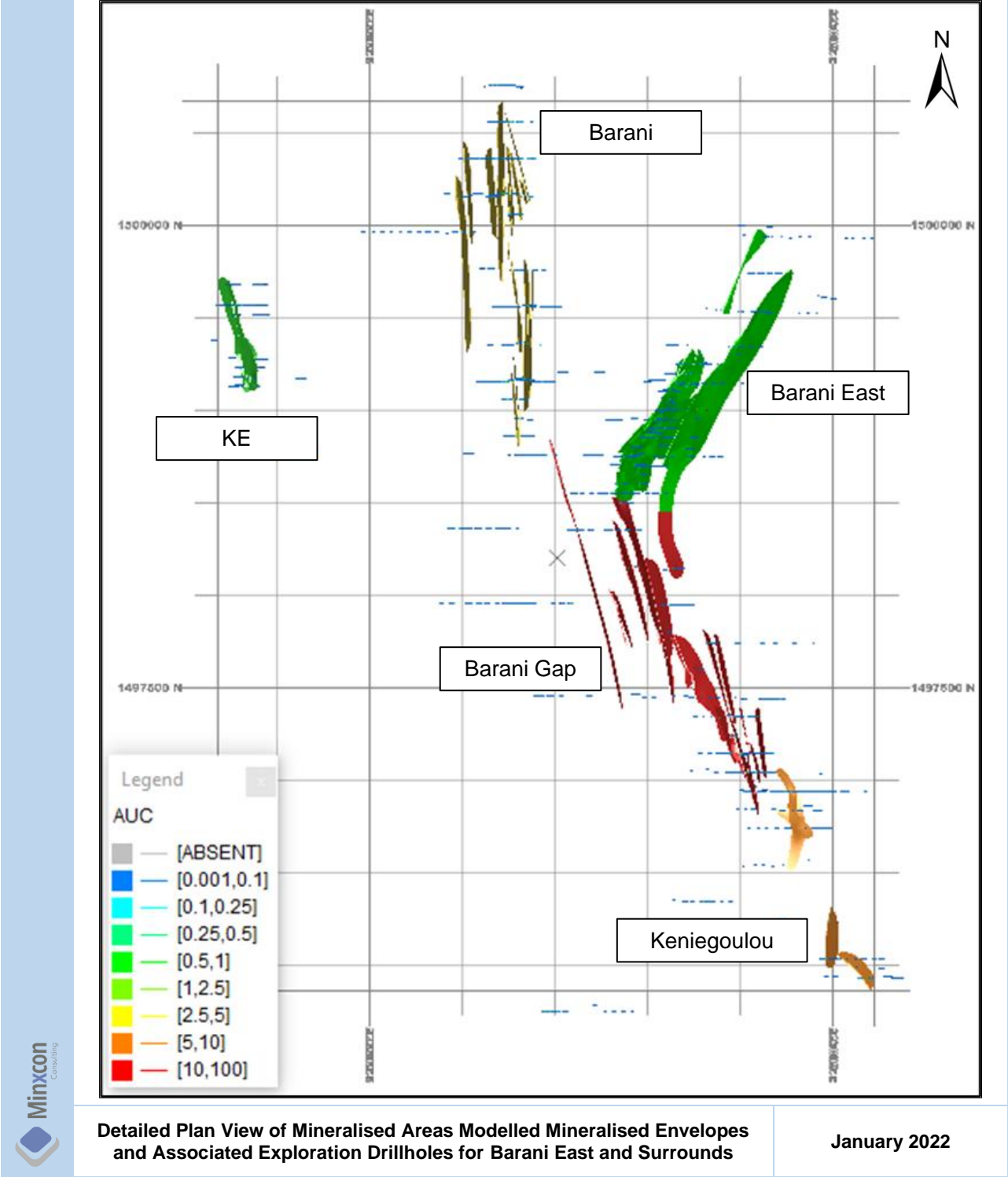
Figure 111: Detailed Plan View of Mineralised Areas Modelled Mineralised Envelopes and Associated Exploration Drillholes for Barani East and Surrounds
