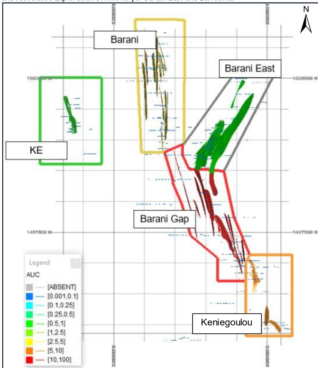
Figure 124: Modelled Geological / Geostatistical Domains of Mineralised Areas Modelled Mineralised Envelopes and Associated Exploration Drillholes for Barani East and Surrounds
