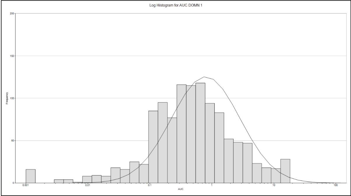
Figure 122: Example of Log Histogram from Barani East
