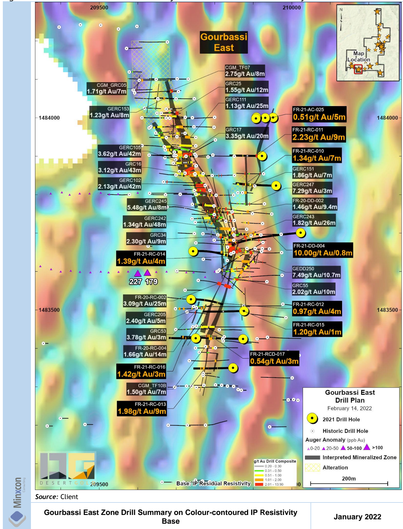
Figure 57: Gourbassi East Zone Drill Summary on Colour-contoured IP Resistivity Base
