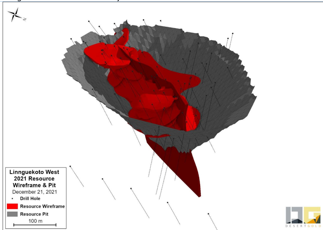
Figure 71: Linnguekoto West Modelled Wireframes and Resource Pit
