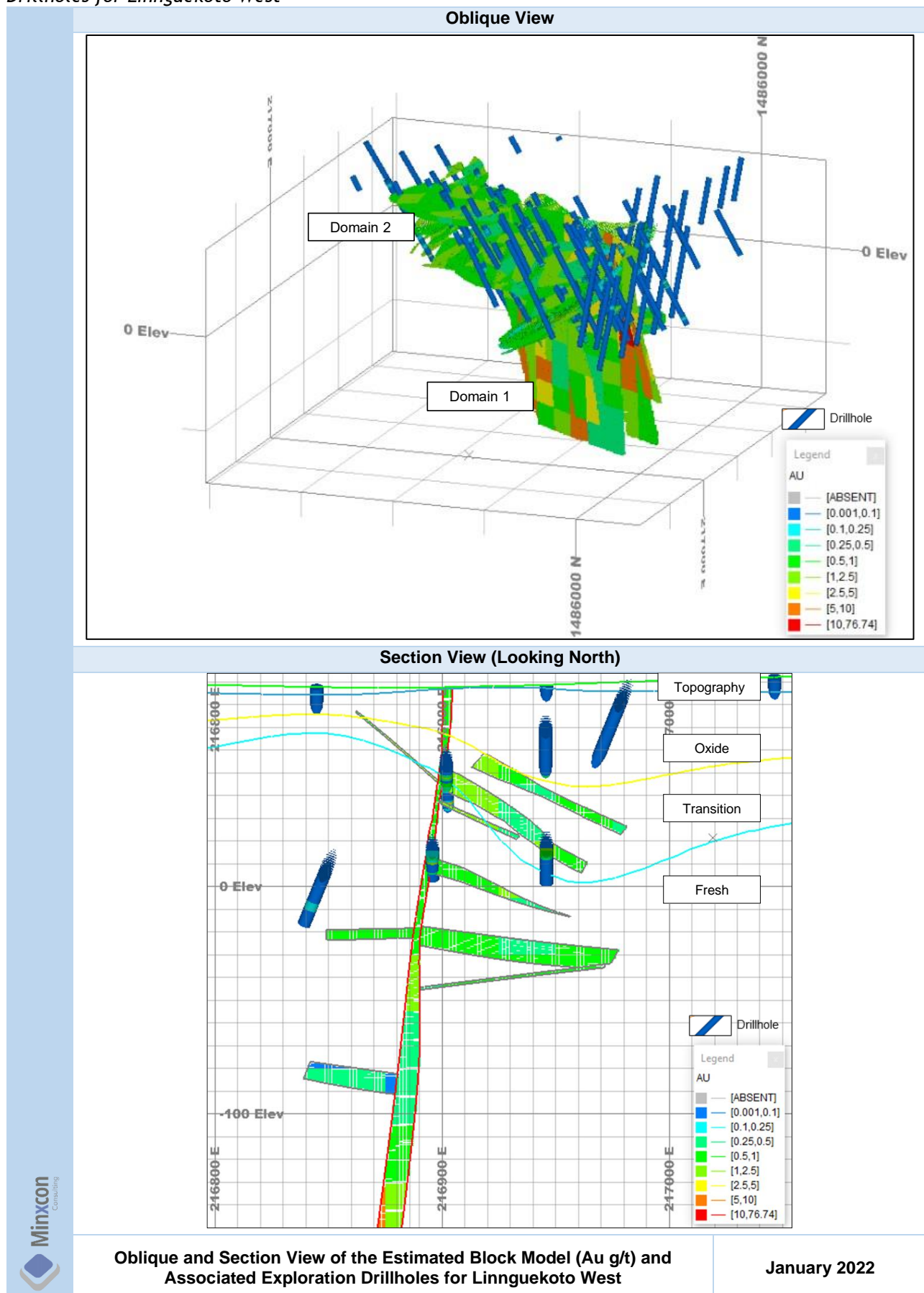
Figure 139: Oblique and Section View of the Estimated Block Model (Au g/t) and Associated Exploration Drillholes for Linnguekoto West
