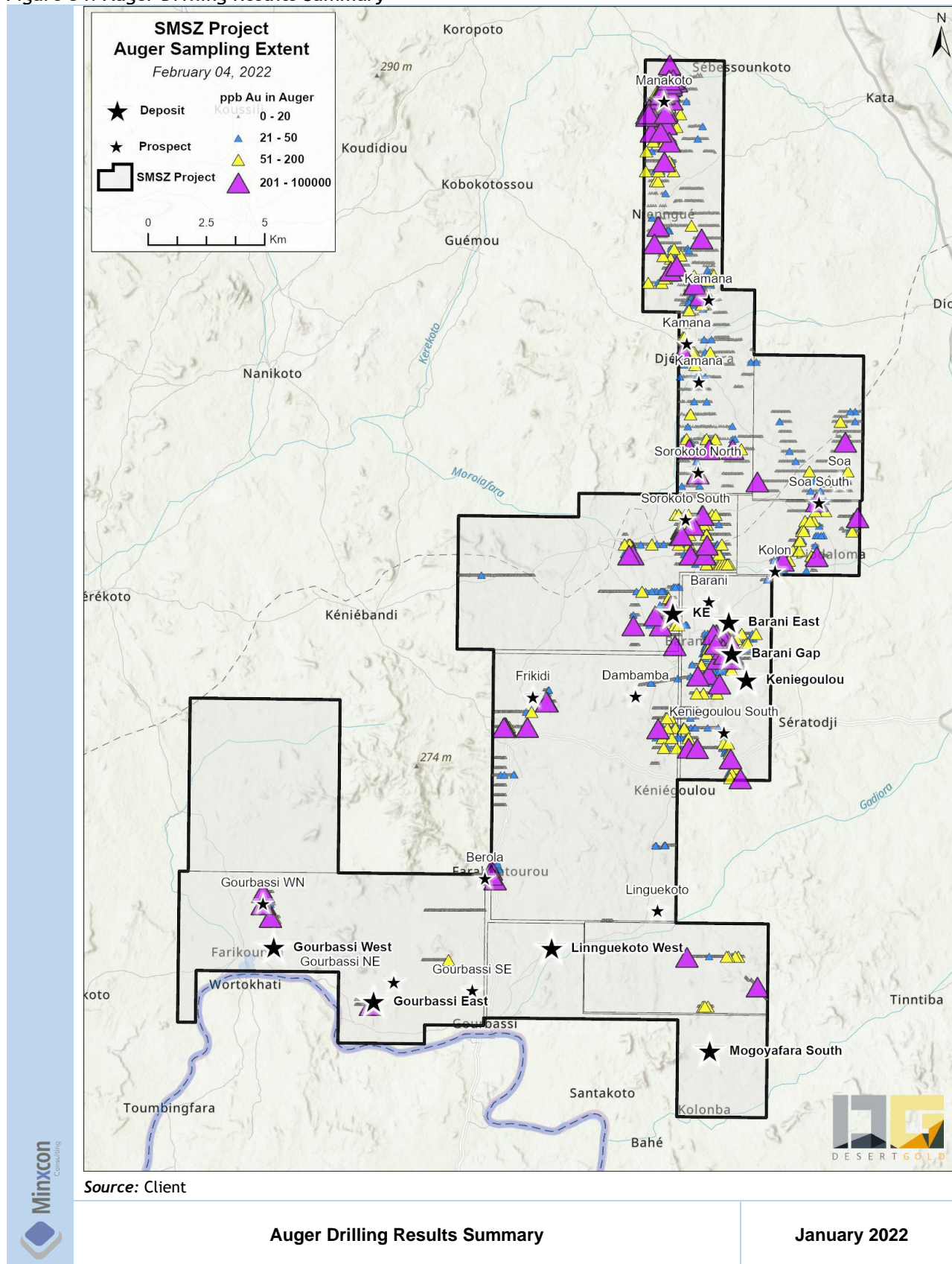
Figure 34: Auger Drilling Results Summary
