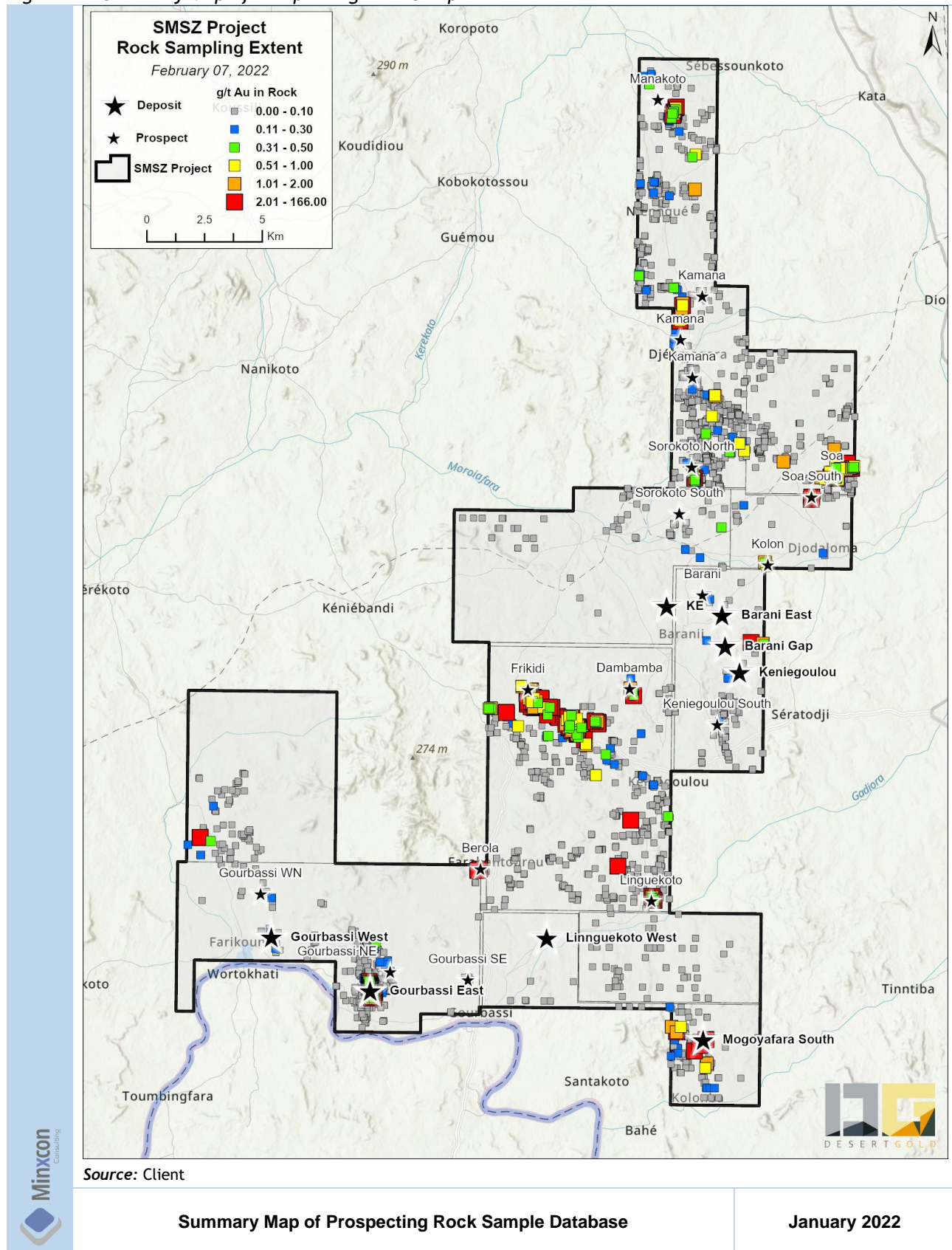
Figure 32: Summary Map of Prospecting Rock Sample Database
