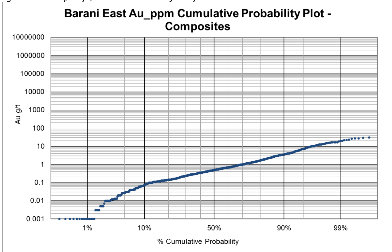
Figure 131: Example of Cumulative Probability Plot from Barani East
