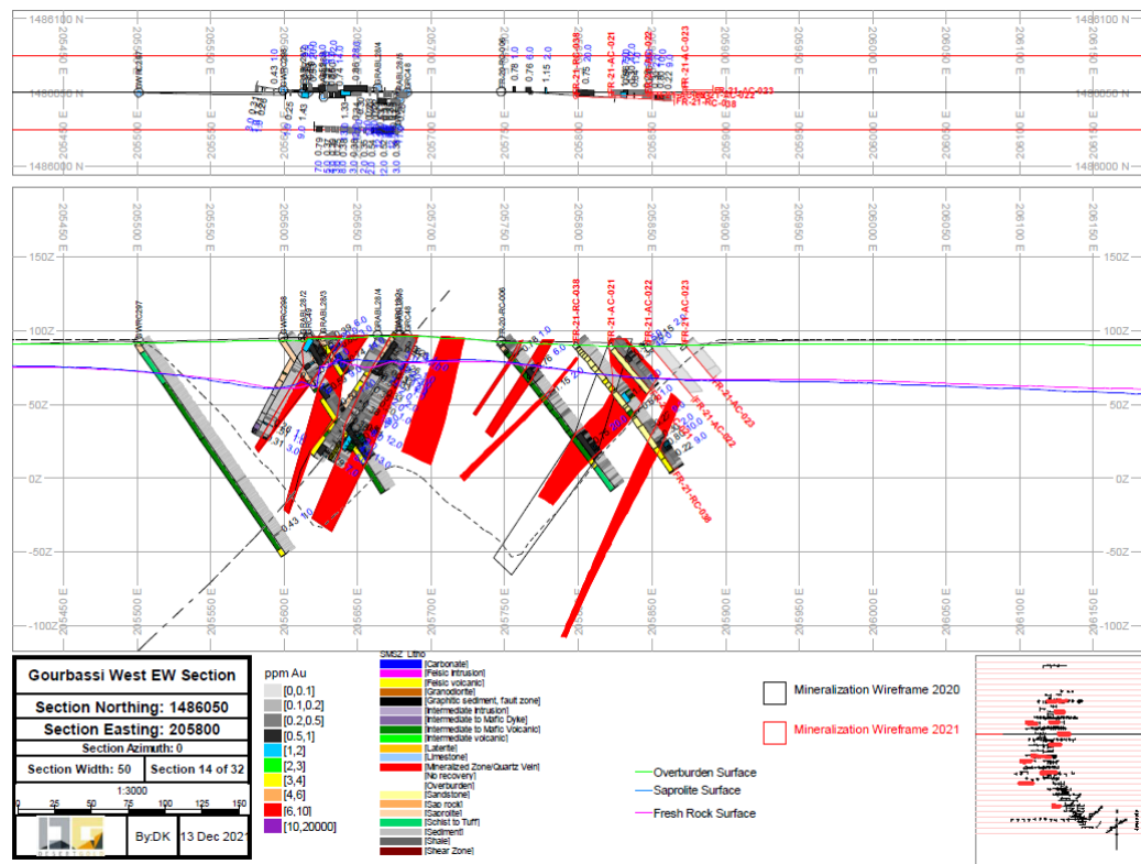
Figure 67: Typical Section through Gourbassi West Deposit
