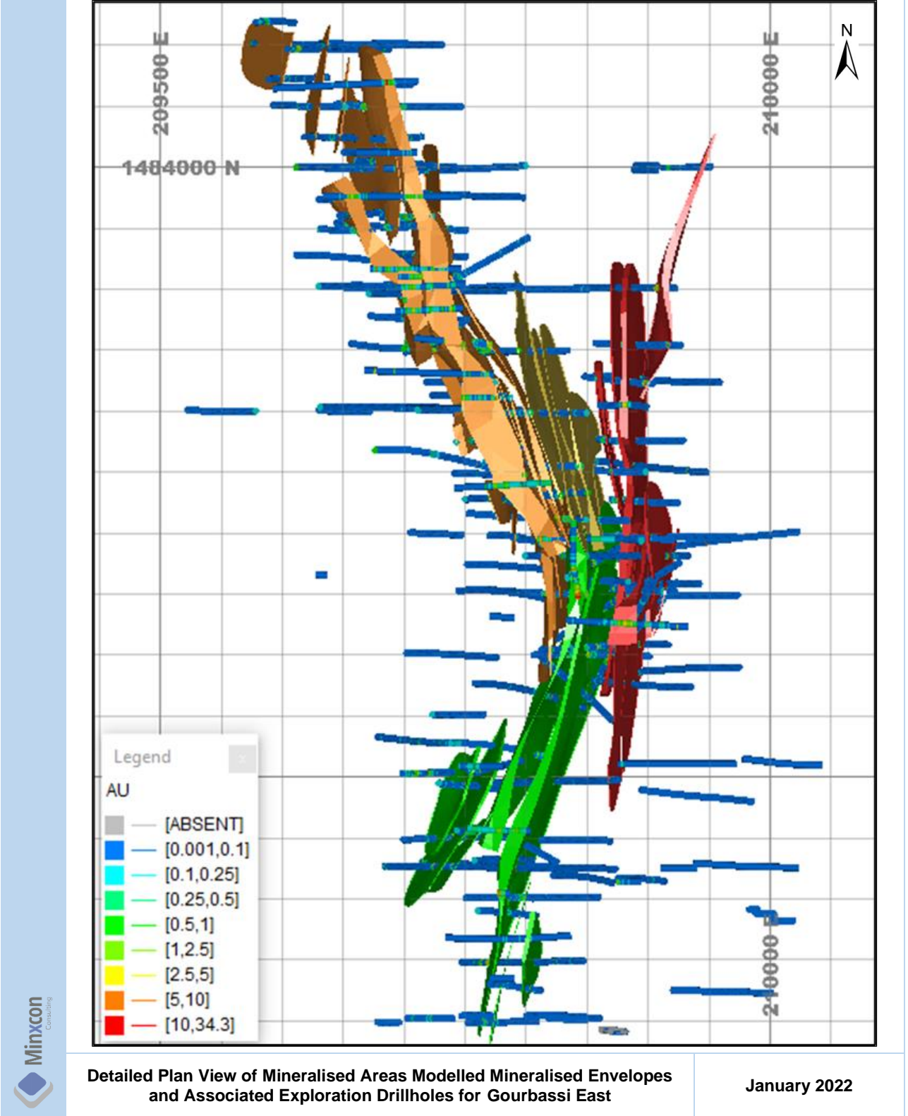
Figure 112: Detailed Plan View of Mineralised Areas Modelled Mineralised Envelopes and Associated Exploration Drillholes for Gourbassi East
