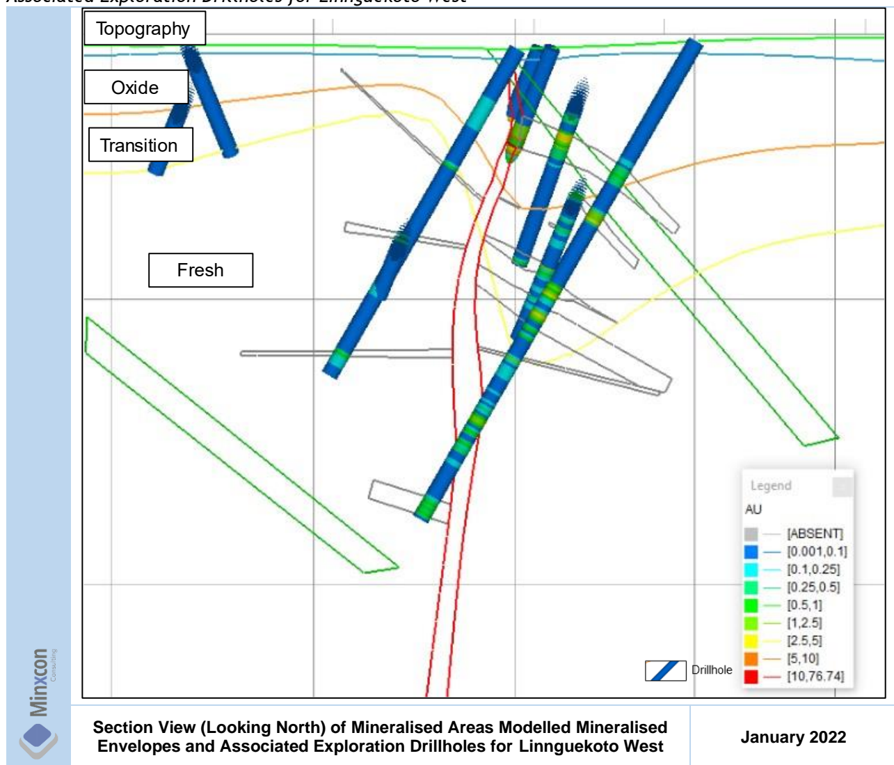
Figure 120: Section View (Looking North) of Mineralised Areas Modelled Mineralised Envelopes and Associated Exploration Drillholes for Linnguekoto West
