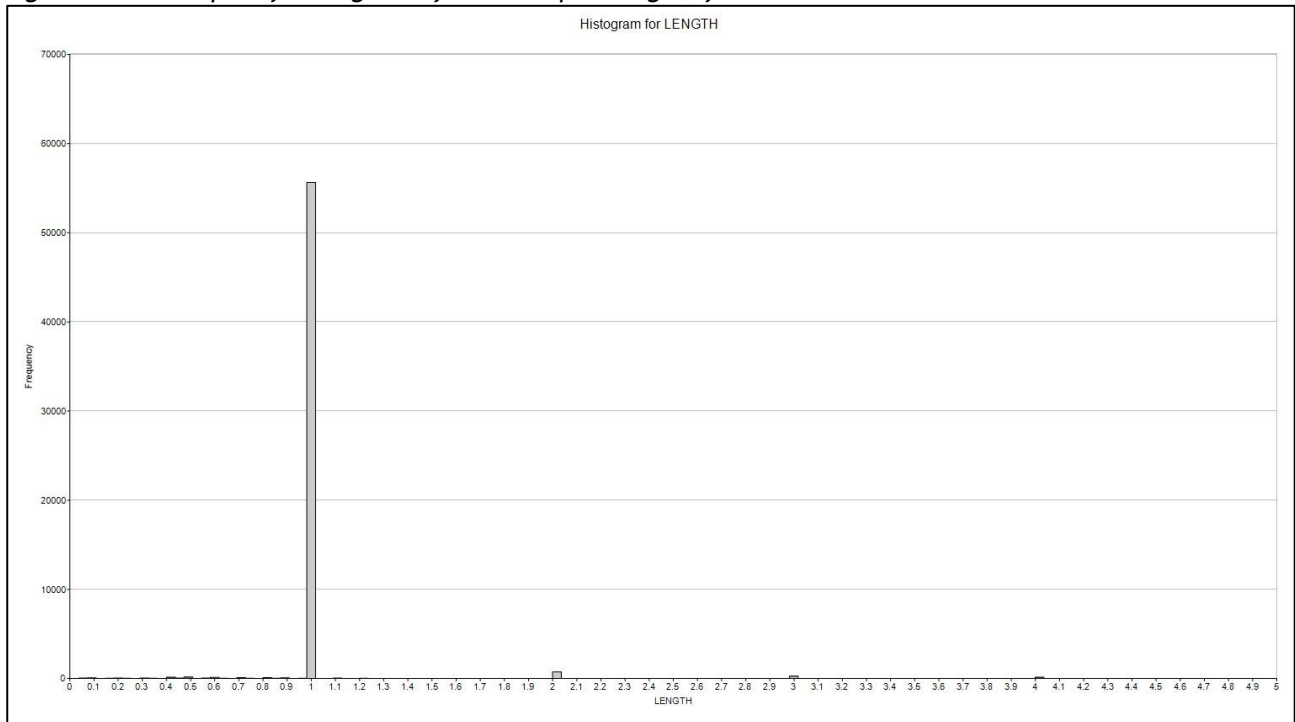
Figure 129: Example of Histogram of Raw Sample Lengths from the Drillhole Data in the Barani Area
